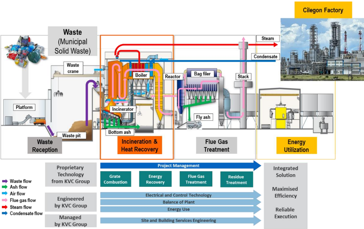
Figure 2.2 Waste to Steam System Configuration Source: Kanadevia, 2026
