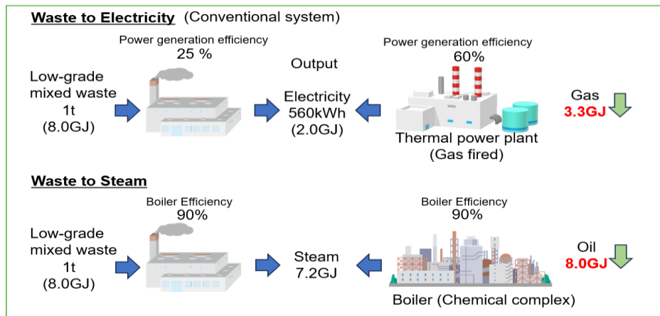
Figure 2.14 High Energy Recovery
