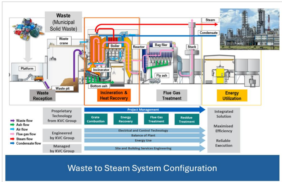
Figure 1.4 Waste to Steam System Configuration
