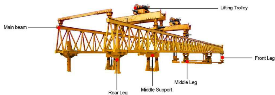
Figure 1.4 Launcher Gantry Parts (Source: Comtec's Manual Book)
