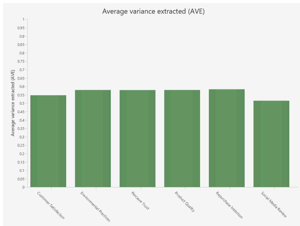
Figure 4.2 AVE Graph
