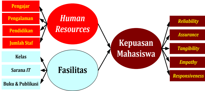
Gambar 16.1 Model Penelitian
