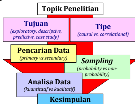
Gambar 16.2 Proses Penelitian
