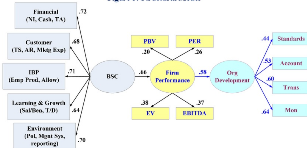
Figure 3: Structural Model
