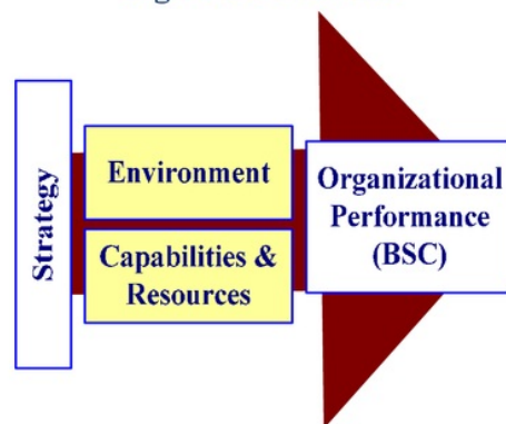
Figure 1: ESC Model
