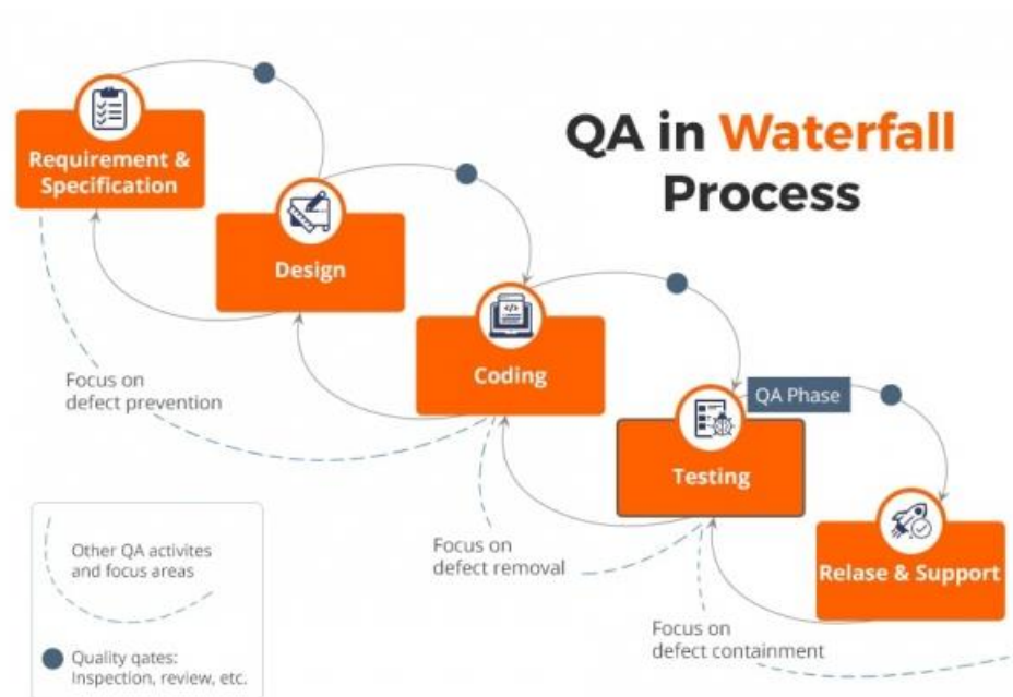
FIGURE 1 WATERFALL PROCEDURE
